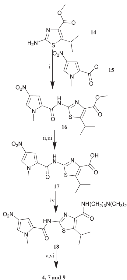
Scheme 2 i) 14 & 15 , NMM, DCM; ii) NaOH aq ; iii) thionyl chloride; iv) 17 & NH 2 (CH 2 ) 3 N(CH 3 ) 2 , HBTU/NMM/DMF; v) Pd/C/H 2 ; vi) HBTU/NMM/DMF, dicarboxylic acid ( 13 , 19 and 20 ).
